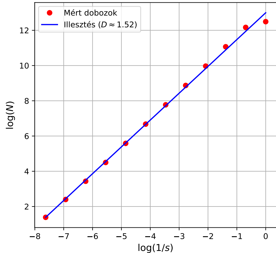
1D automata (rule 90)
